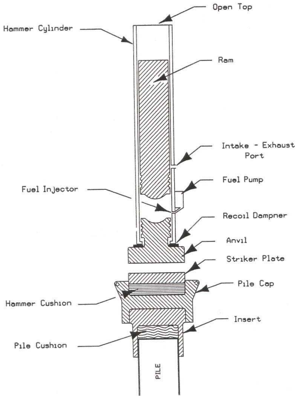
SINGLE ACTING DIESEL HAMMER
